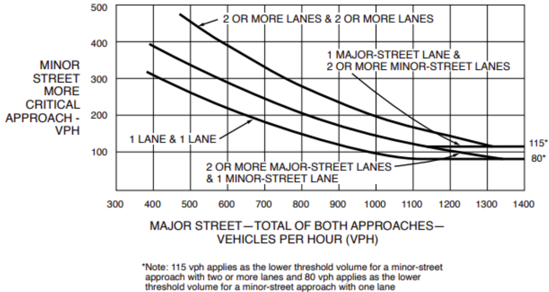
Figure 5-8: Warrant 2, Four-Hour Vehicular Volume, Manual on Uniform Traffic Control Devices for Streets and Highways, 11 th Edition (2023)
