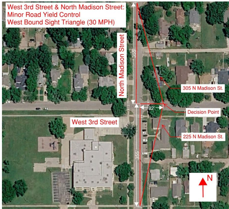
3 rd & Madison - Yield Control Westbound Sight Distance
