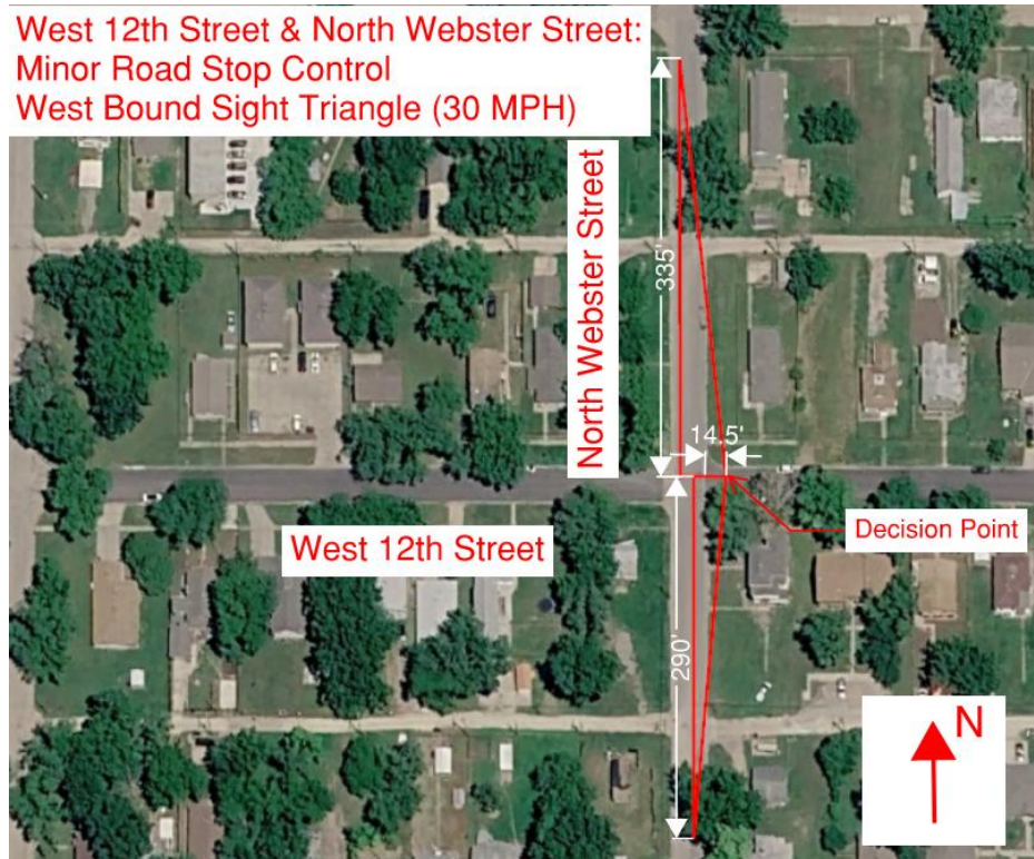
12 th & Webster - Two-Way Stop Control Westbound Sight Distance
