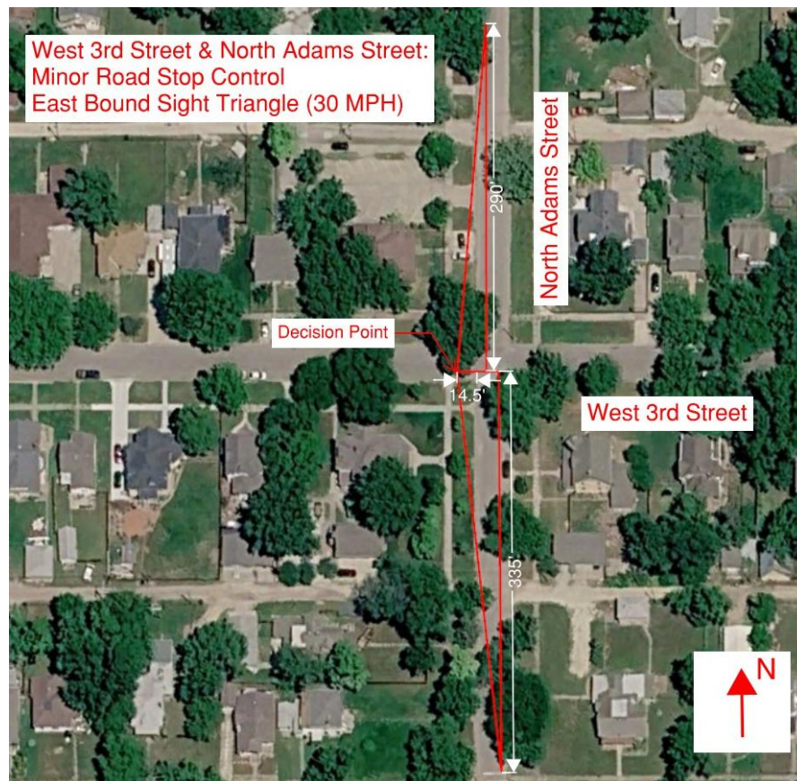
3 rd & Adams - Two-Way Stop Control Eastbound Sight Distance
