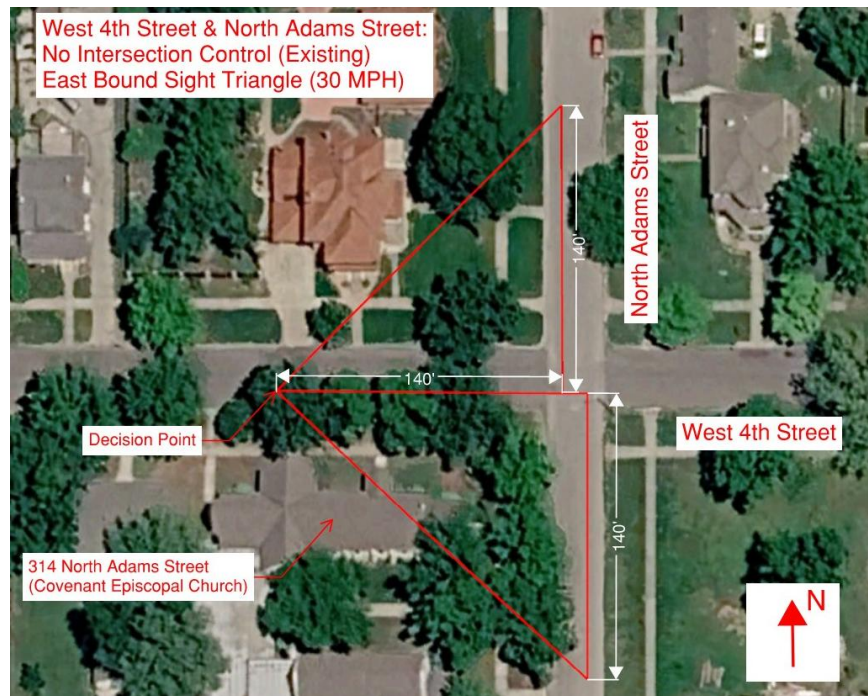
4 th & Adams - No Intersection Control Eastbound Sight Distance
