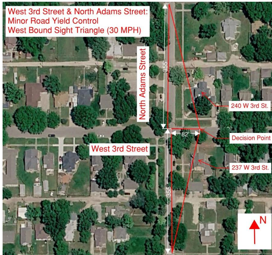
3 rd & Adams - Yield Control Westbound Sight Distance
