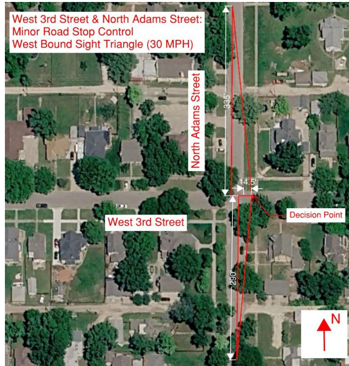
3 rd & Adams - Two-Way Stop Control Westbound Sight Distance
