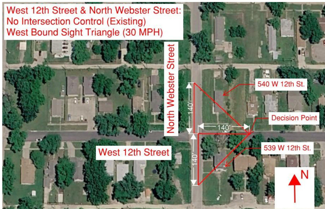
12 th & Webster - No Intersection Control Westbound Sight Distance
