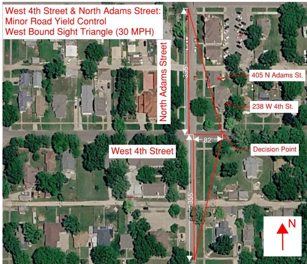
4 th & Adams - Yield Control Westbound Sight Distance
