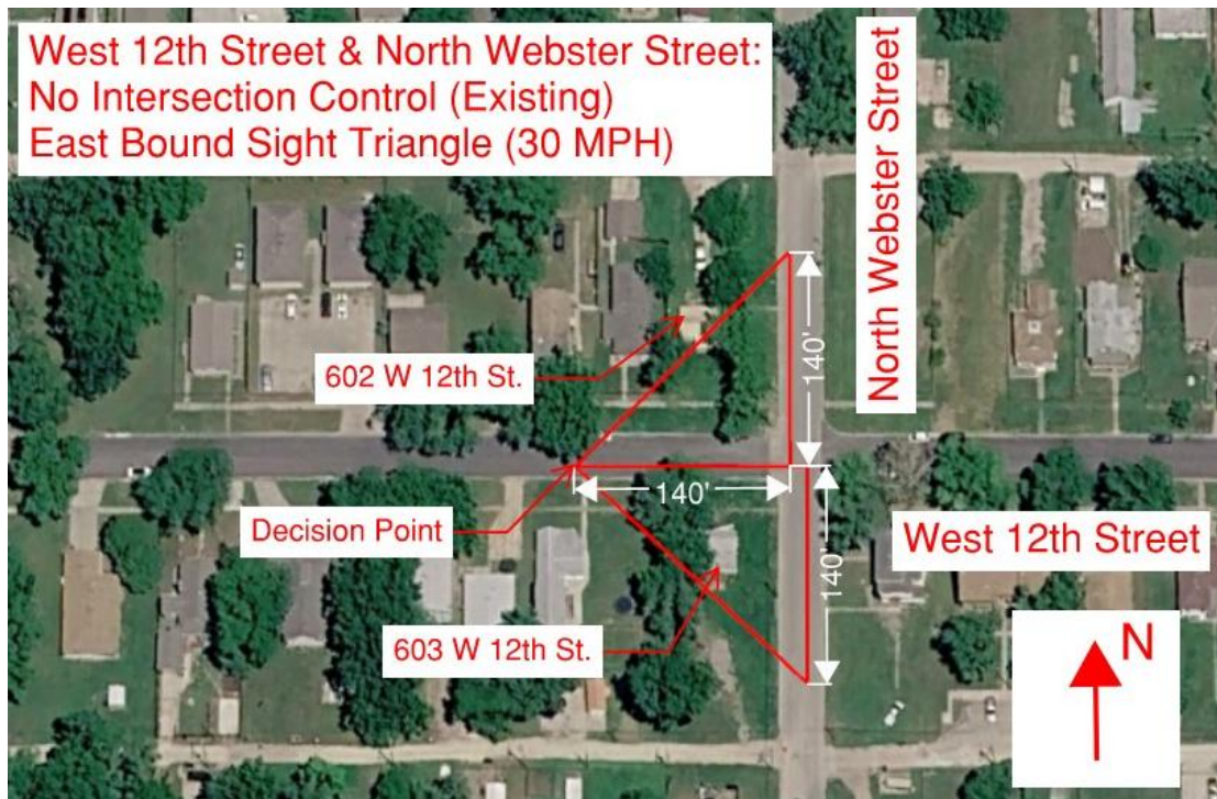
12 th & Webster - No Intersection Control Eastbound Sight Distance
