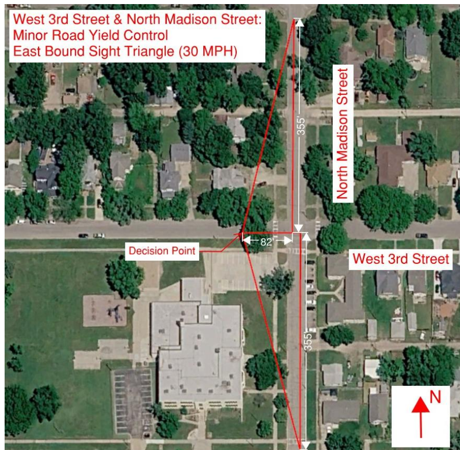
3 rd & Madison - Yield Control Eastbound Sight Distance
