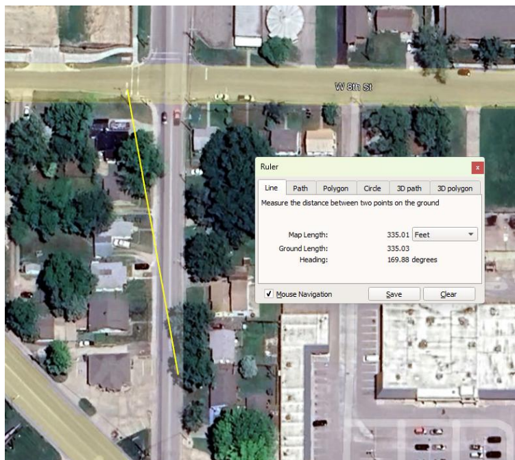
Figure 5-6: East Bound Sight Distance
