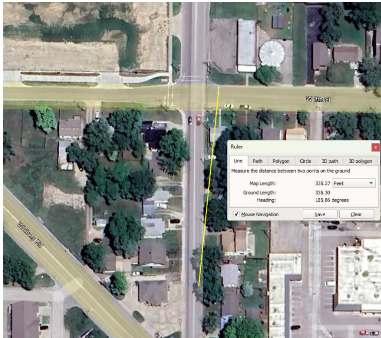
Figure 5-5: West Bound Sight Distance
