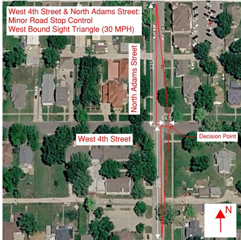
4 th & Adams - Two-Way Stop Control Westbound Sight Distance
