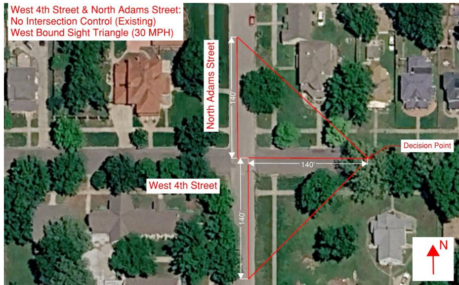
4 th & Adams - No Intersection Control Westbound Sight Distance
