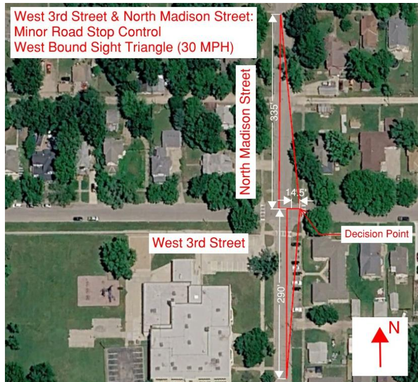
3 rd & Madison - Two-Way Stop Control Westbound Sight Distance
