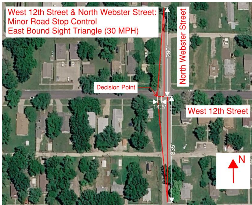
12 th & Webster - Two-Way Stop Control Eastbound Sight Distance
